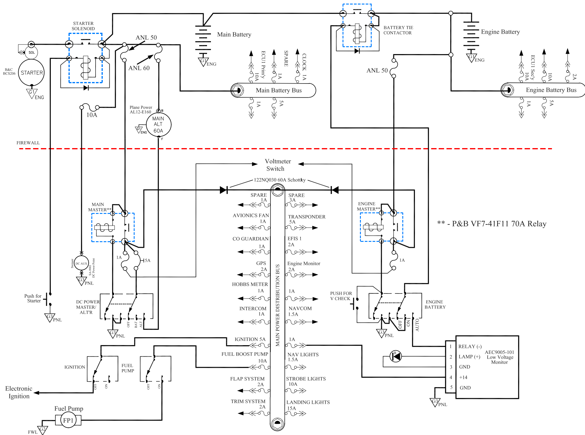
DUAL BATTERY ELECTRICAL SYSTEM
