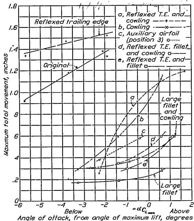
FIGURE 27.—Amplitude of stabilizer-tip movements under various conditions. Angle of attack corrected for tunnel effects. Power off. Air speed approximately 58 m.p.h.
