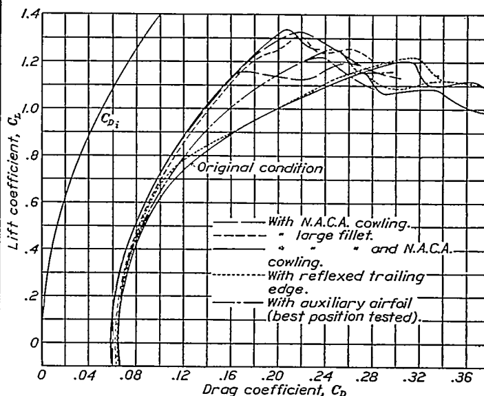
FIGURE 17.—Polars for McDonnell airplanes comparing various devices. Corrected for tunnel effects. Power off.
