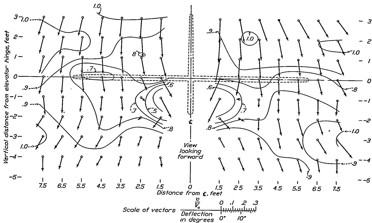
FIGURE 32.—Air flow at tail of McDonnell airplane with N.A.C.A. cowling, power off. Survey in vertical plane through elevator hinge line. The contours show the ratio of the dynamic pressure behind the airplane to the dynamic pressure in the free air stream. The vectors show the components of the velocity in the plane of the survey. Angle of attack (thrust axis) = 13.9^\circ (corrected for tunnel effects). Lift coefficient = 1.153.
