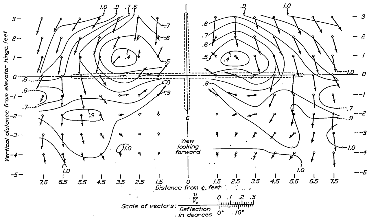
FIGURE 29.—Air flow at tail of McDonnell airplane in original condition, power off. Survey in vertical plane through elevator hinge line. The contours show the ratio of the dynamic pressure behind the airplane to the dynamic pressure in the free air stream. The vectors show the components of the velocity in the plane of the survey. Angle of attack (thrust axis) =14.2^\circ (corrected for tunnel effects). Lift coefficient =0.984 .
