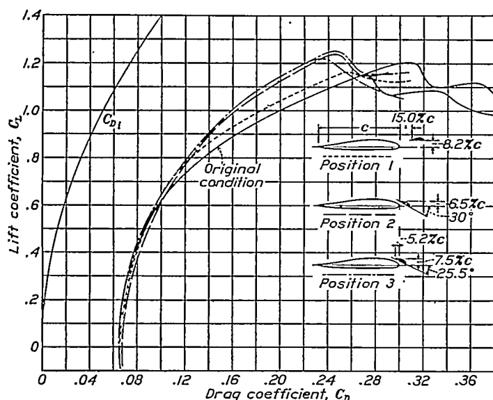
FIGURE 15.—Polars for McDonnell airplanes with auxiliary airfoils. Corrected for tunnel effects. Power off.
