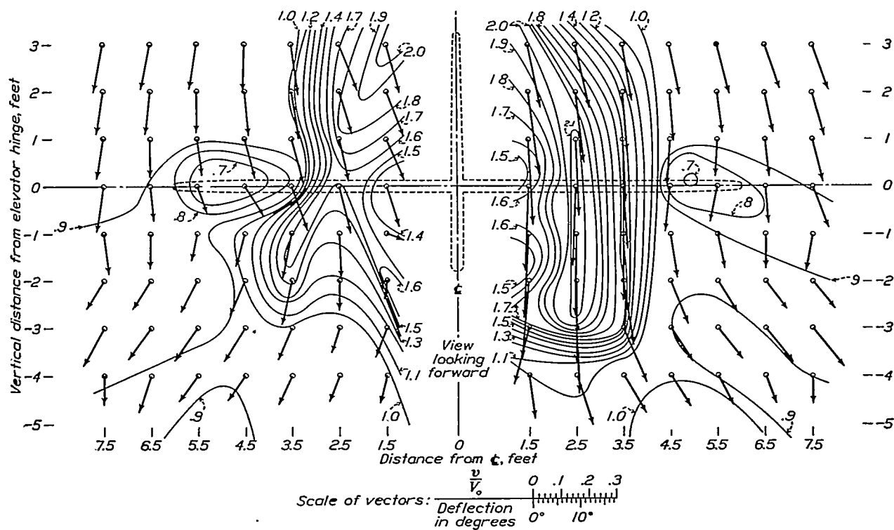
FIGURE 33.—Air flow at tail of McDonnell airplane in original condition, power on. Survey in vertical plane through elevator hinge line. The contours show the ratio of the dynamic pressure behind the airplane to the dynamic pressure in the free air stream. The vectors show the components of the velocity in the plane of the survey. Angle of attack (thrust axis) = 13.7^\circ (corrected for tunnel effects). Lift coefficient = 1.241.
