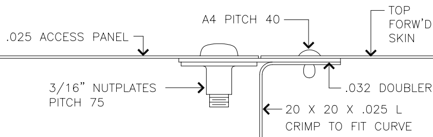
SECTION "B"
